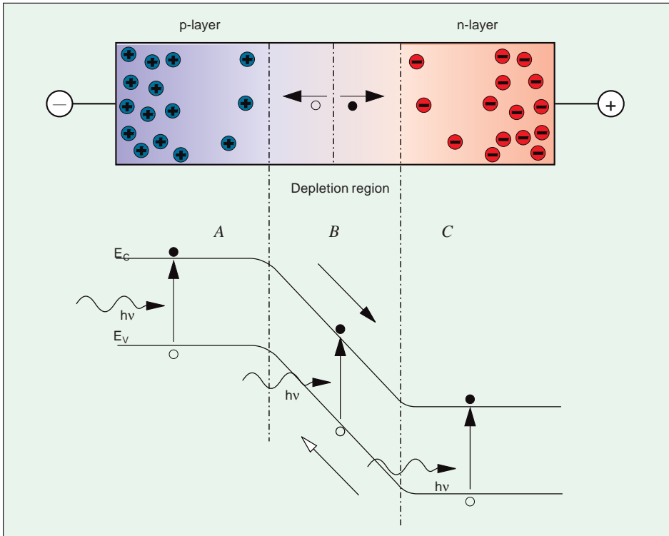
Fig. 7-2 An incident photon can cause the production of e-h pairs in three different regions (A, B and C) in the p-n diode. However, rapid detection is only achievable in B, the depletion region.
