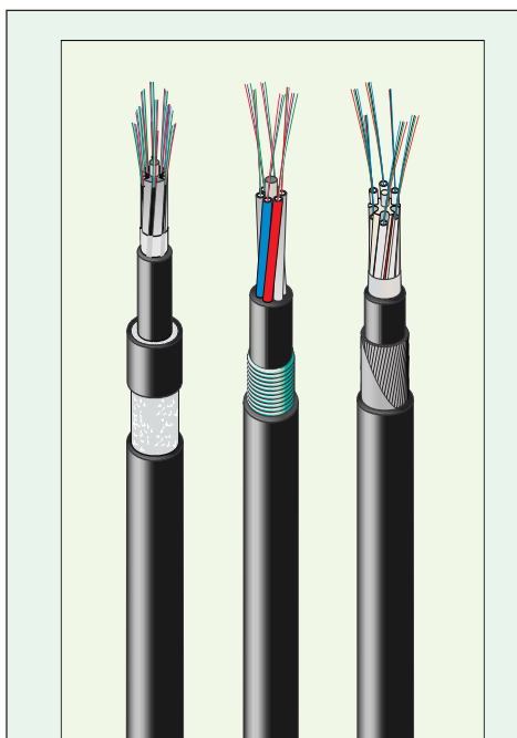
Fig. 11-4 Three typical samples of cables made for direct burial. Left is the HET-reinforced GASLLDV perfect for laying along electrified railroads. In the middle is the GRHLWLV for lighter ground and to the right is GRSLTLV for rough terrain.
