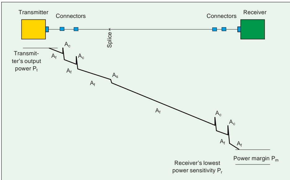
Fig. 9-5 Example 1: The constituent components and the OTDR curve, which shows the attenuation in the fiber optic link from transmitter to receiver.
