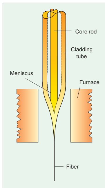
Fig. 12-4 Fiber fabrication by "rod in tube" method.
