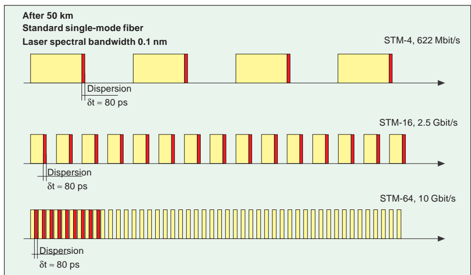
Fig. 9-11 Chromatic dispersion for a standard single-mode fiber after 50 km. The chromatic dispersion is 16 ps/nm×km. The spectral bandwidth of the transmitting laser is set to 0.1 nm. Only the STM-64 will fail.
