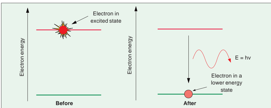
Fig. 6-17 Spontaneous emission.
