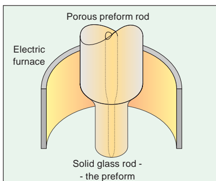
Fig. 3-8 The porous preform is collapsed into a solid glass rod.
