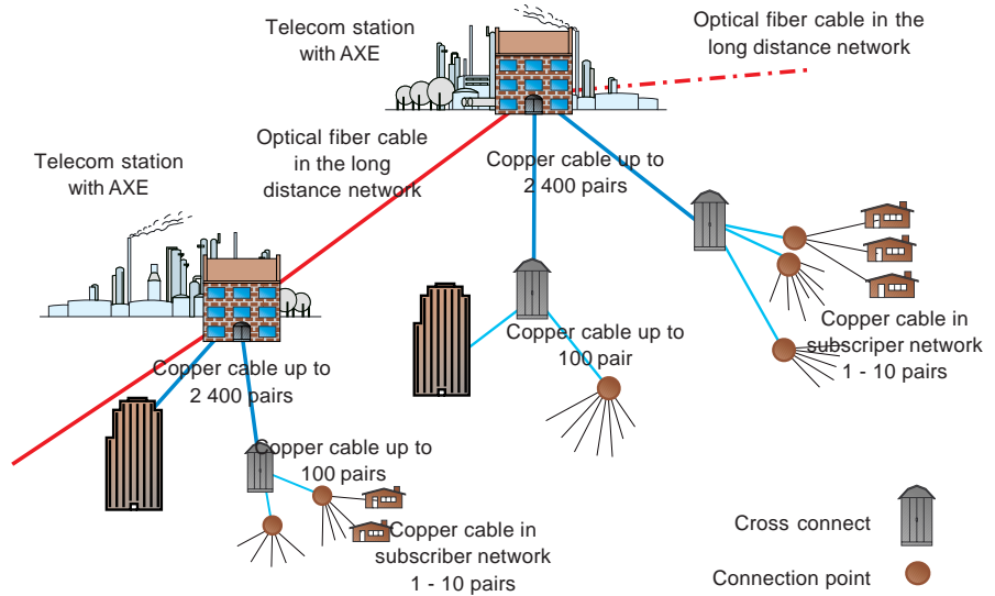
Fig 1-12. Traditional telecom network based on optical fiber cables between telecom stations and copper cables from station to subscriber.
