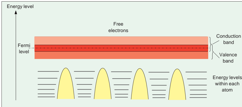
Fig. 6-10 In a conductor, the valence and conduction bands run into each other and only a small addition of energy is needed to move electrons from atom to atom.
