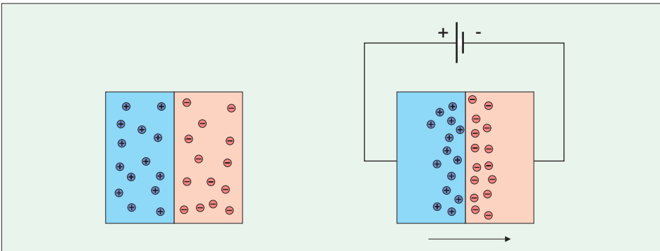
Fig. 6-19 With a forward-biased voltage, an accumulation of electrons and holes is obtained at the junction between the p- and n-layers.
