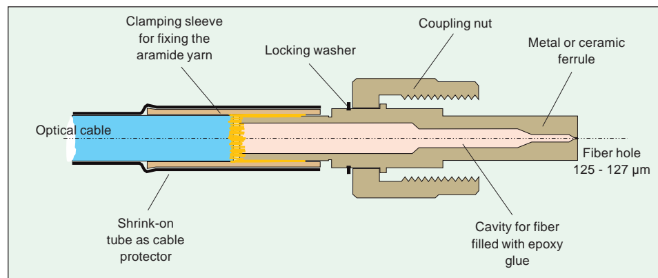
Fig. 8-8 An SMA connector in cross-section.
