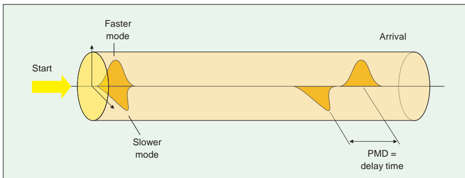
Fig. 4-8 Pulse broadening through polarization mode dispersion, PMD.
