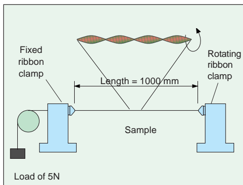
Fig. 5-12 Setup for torsion test.
