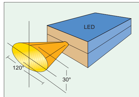
Fig. 6-30 The radiation lobe is an ellipse with an opening of around 115 - 125^\circ in horizontal direction and 25 - 35^\circ in vertical direction.
