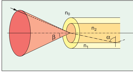
Fig. 4-3 The acceptance cone of a fiber.
