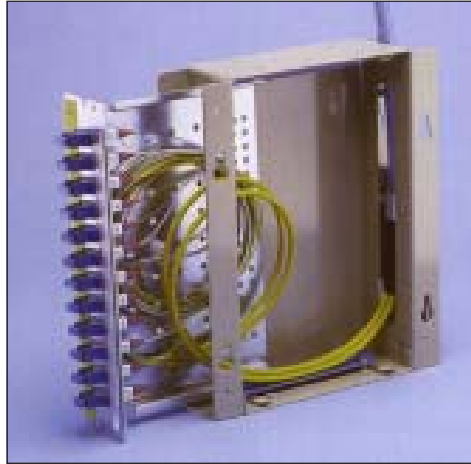
itself can be designed as a separate unit. Fig. 11-48 Pre-terminated line terminal or termination unit
