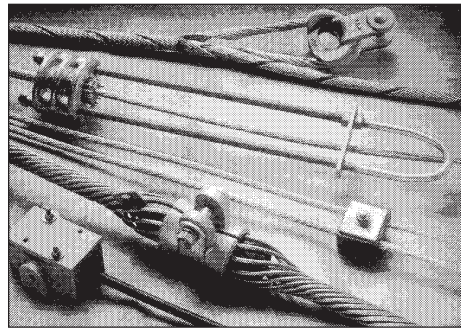
Fig. 11-22 Guy-grips and different cable fixing devices
