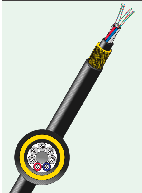
Fig. 5-35 Aerial cable with a large amount of of aramide yarn as strength member. This type of cable is self supporting for spans up to 1 000 m. Cable illustrated is the Skyspan™ (Focas Inc.).
