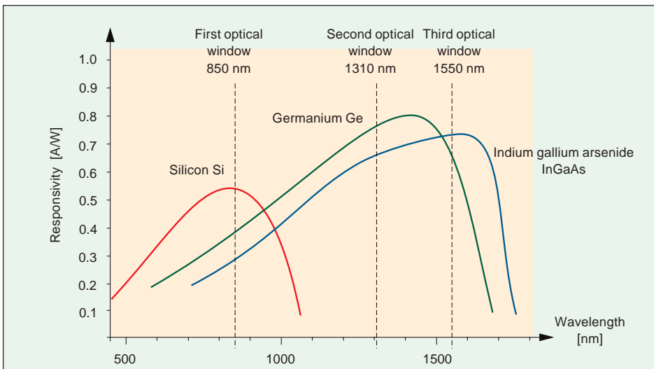
Fig. 7-10 The responsivity of a photodiode is dependent both on the wavelength of the incident light and the materials used.
