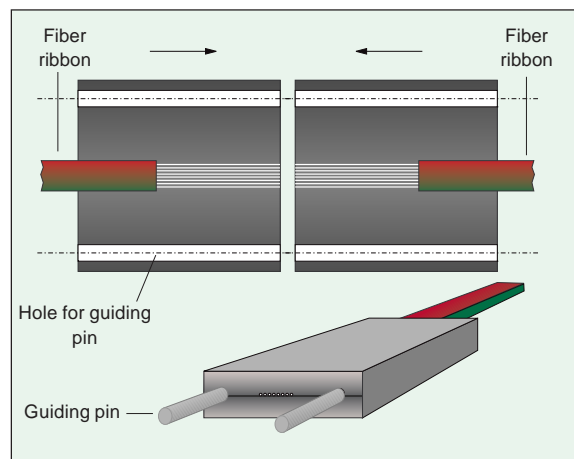
Fig. 8-39 Schematic diagram of a splice for a fiber ribbon
