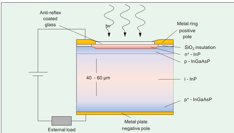
Fig. 7-9 Construction of an RAPD.
