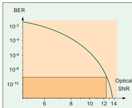
Fig. 7-12 Relationship between BER and optical SNR.
