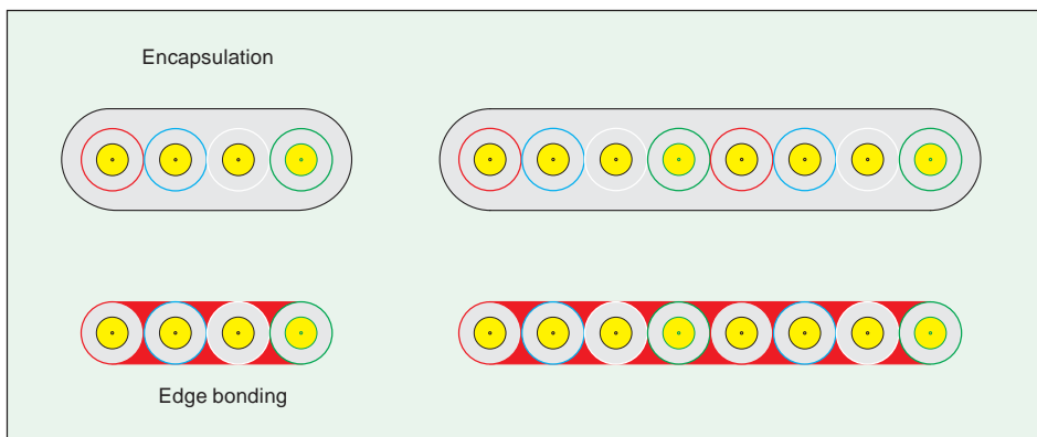
Fig. 5-9 The three most common methods of manufacturing fiber ribbon.
