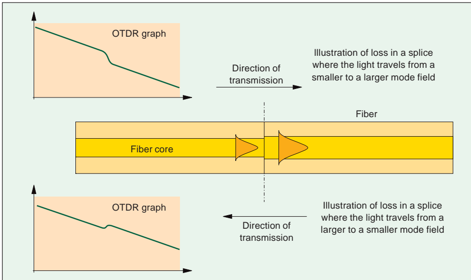
Fig. 8-2 Loss measurements in optical fiber networks - at splices between fibers with mode fields of different sizes - can give unexpected values.
