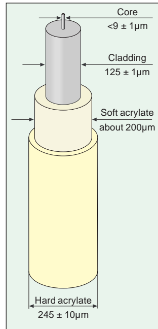
Fig 3-13 Typical primary coated single-mode fiber.
