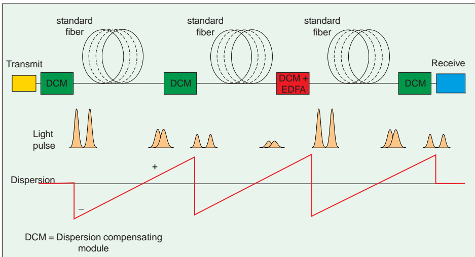
Fig. 4-18 The dispersion compensating modules can be used at the beginning, in the middle or at the end of a transmission link. They can preferably be combined with an EDFA.
