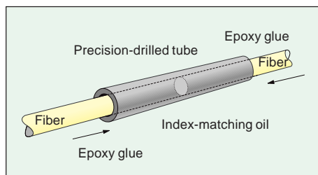
Fig. 8-21 The fibers are pushed from either end into a precision-drilled tube.
