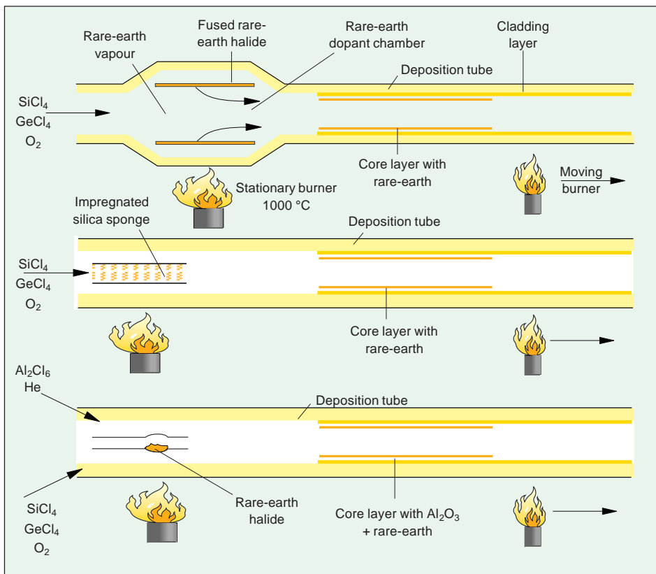
Fig. 12-6 Various forms of the “volatile halide” method.
