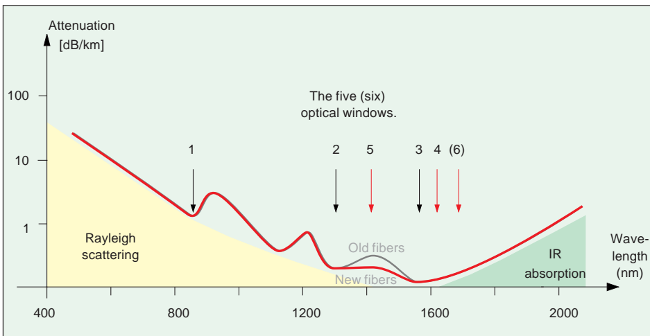
Fig. 2-3 The attenuation curve for optical fiber (glass). Note the five optical wavelength windows.
