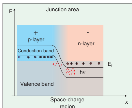
Fig. 6-21 A forward biased p-n junction. The current flowing through the device causes a large number of electrons to recombine with the holes in the junction area, and loose their excess energy as light quanta, photons.
