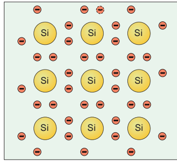
Fig. 6-13 The structure of a silicon crystal, where the outermost electrons of each atom are “shared” so that a full outer shell is formed.
