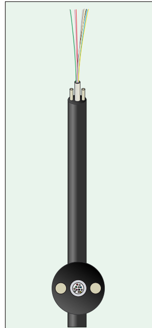
Fig. 5-41 Outdoor cable with loose tube suited for FTTH etc.
