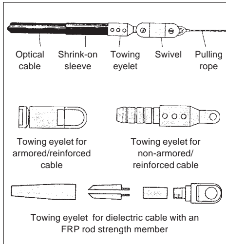
Fig. 11-10 Different types of installation device.
