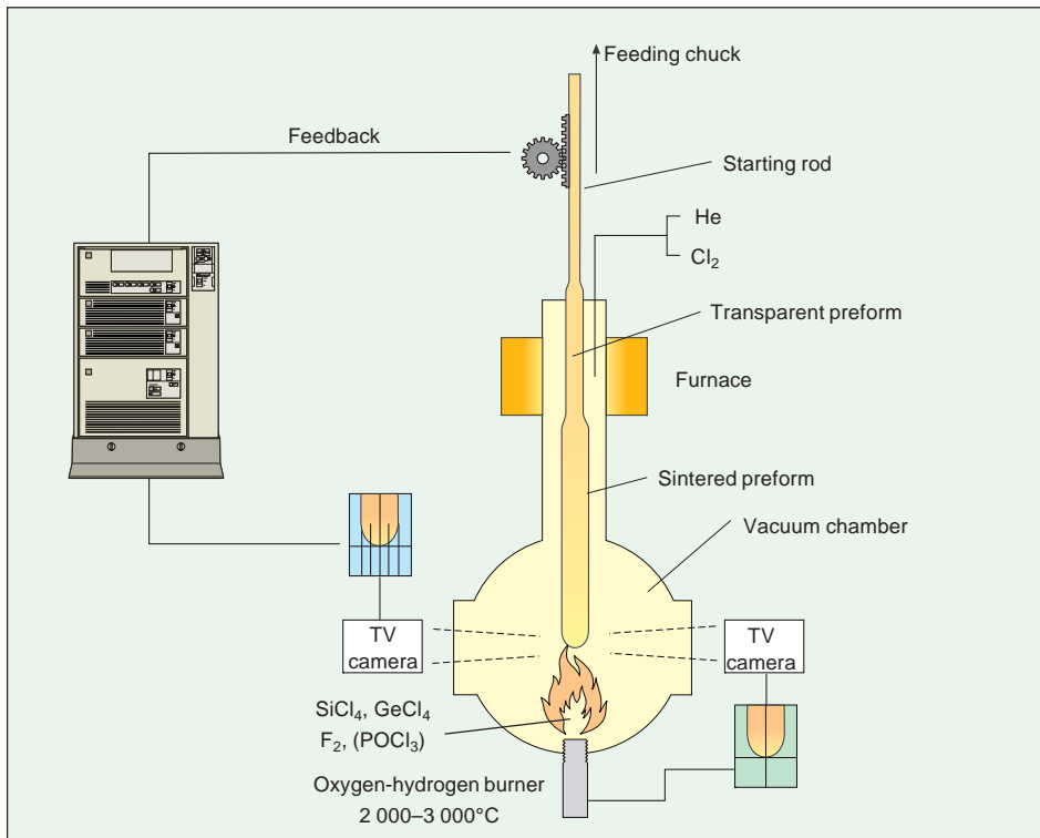
Fig. 3-10 Schematic diagram showing the VAD method of preform manufacture.
