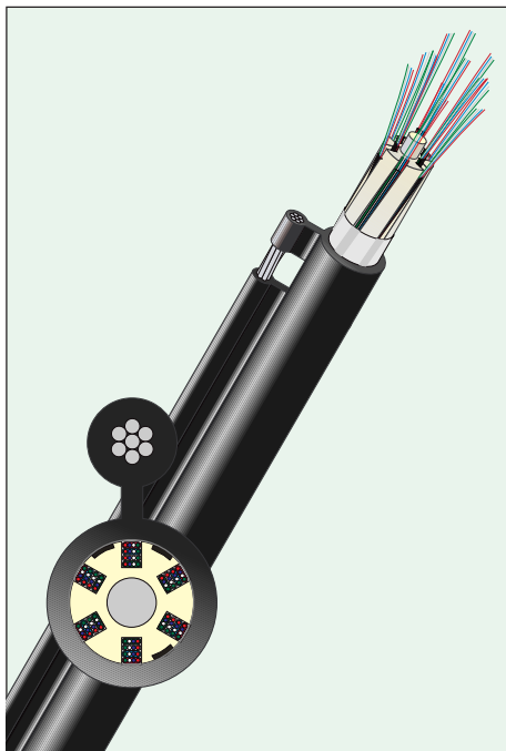
Fig. 5-36 With a steel suspension strand, optical fiber cable can be suspended in spans of 50 - 70 m. The cable illustrated is GASLCV.
