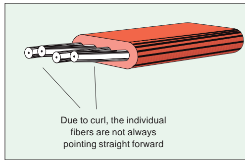
Fig.5-16 Fiber curl.
