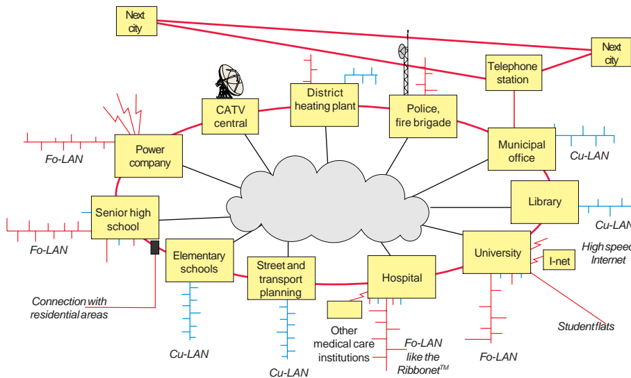
Fig 1-15. Sketchy drawing of an optical fiber community access network
