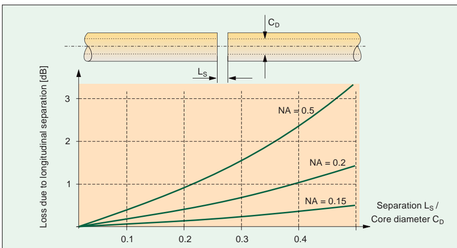
Fig. 8-10 Graph of loss caused by longitudinal separation.
