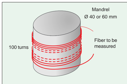
Fig. 5-11 Setup for macrobend test.
