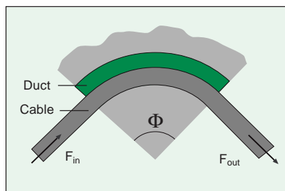
Fig 11-14 Illustration of pulling forces through a bend
