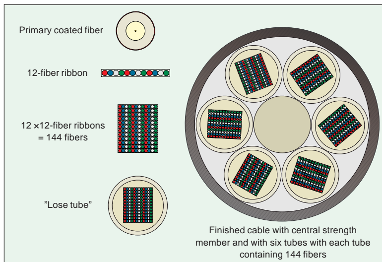
Fig. 5-43 Ribbon cable with 864 fibers
