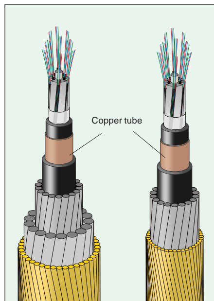
Fig. 5-30 Copper plate formed to a tube and electrically welded to a water-proof encapsulation.
