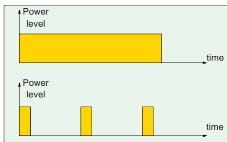
Fig. 10-10 The light from a stabilized light source is often continuous (upper graph), while the light from an OTDR is pulsed (lower graph).
