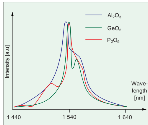
Fig. 12-8 Effect of co-dopant composition on fluorescence spectrum.
