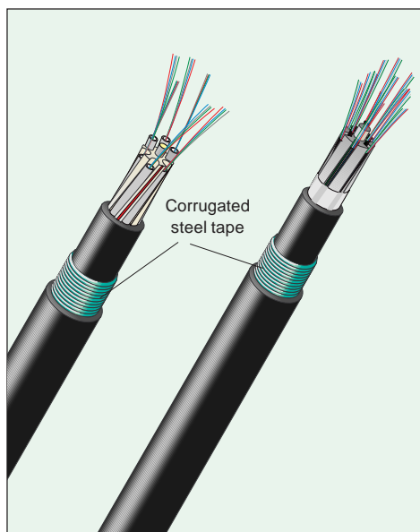
Fig. 5-31 Corrugated steel tape-reinforced cable for laying underground, or in ducts. The cables illustrated are GRSLWLV and GASLWLV.
