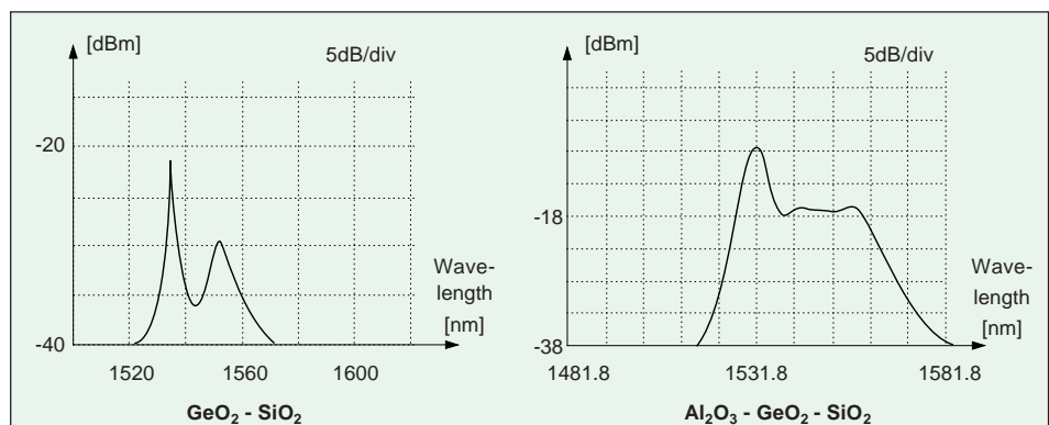
Fig. 12-3 Amplified spontaneous emission of Er^{3+} in different host materials: GeO_2 - SiO_2 to the left and Al_2O_3 - GeO_2 - SiO_2 to the right.
