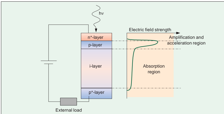
Fig. 7-8 Example of the distribution of field strength in an APD among the different layers.
