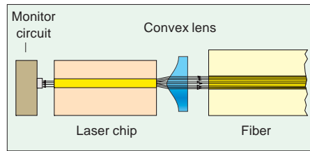
Fig. 6-26 With the help of a microscopically small lens, the light is converged from the laser diode into the fiber.
