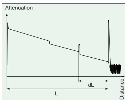
Fig. 10-4 OTDR curve and how it is used for distance measurement.
