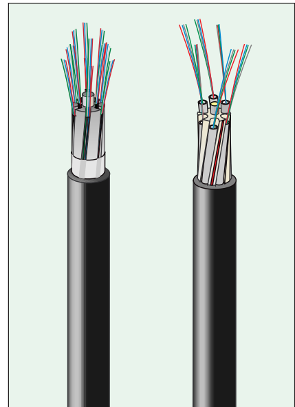
Fig 11-6 Two duct cables the can be used for direct burial installation if precautions are taken, GASLDV and GRSLDV.
