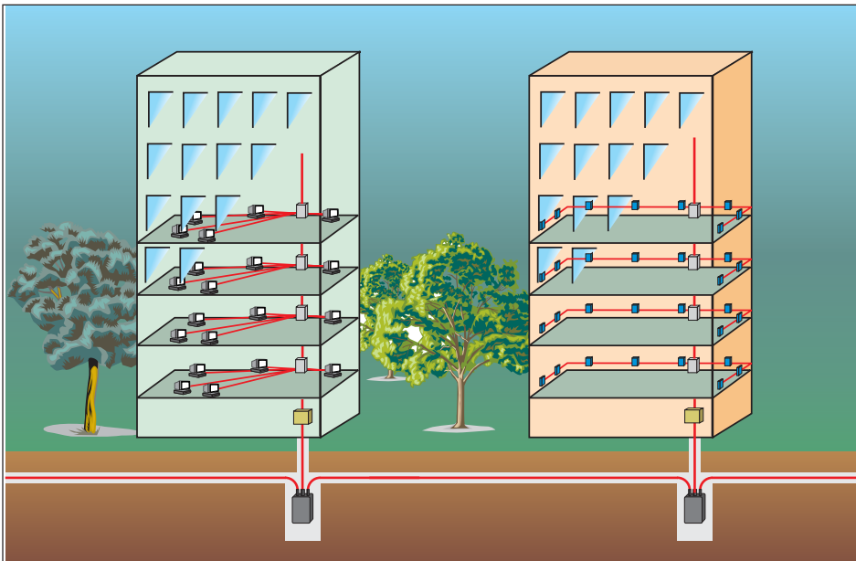
Fig. 11-32 Traditional indoor cabling. To the left is a starlike network shown and to the right is a bus network. Trunk cable to each floor and plenum cable to the user.
