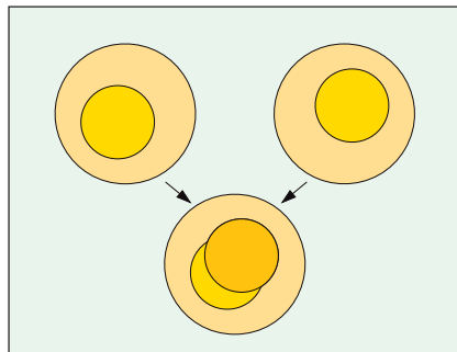
Fig. 8-7 Core/cladding non-concentricity can increase losses.
