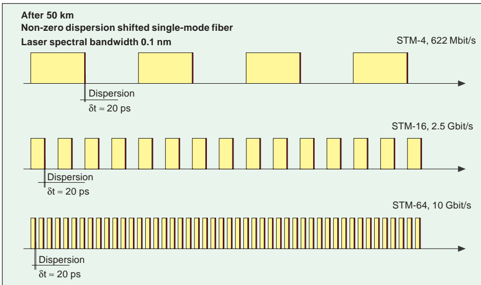
Fig. 9-12 Chromatic dispersion for a non-zero dispersion shifted single-mode fiber after 50 km. The chromatic dispersion is 4 \text{ ps/nm} \times \text{km} . The spectral bandwidth of the transmitting laser is set to 0.1 \text{ nm} . All the three systems will function properly.
