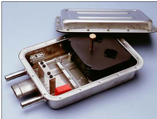
Fig. 11-44 Joint closure NCD 503 all in acid-proof stainless steel.
