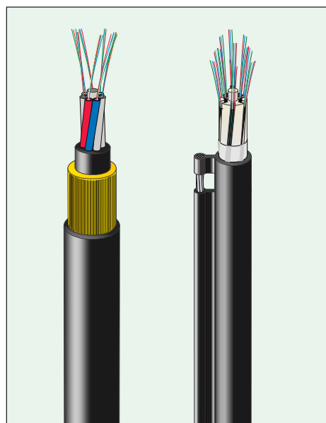
Fig. 11-25 Two samples of self-supporting aerial cable. To the left is a dielectric self-supporting cable and to the right is a cable utilizing a suspension wire.
