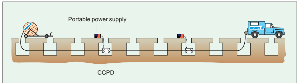
Fig. 11-12 The use of CCDPs (Caterpillar Capstans Pulling Devices) in the laying of long cable sections.
