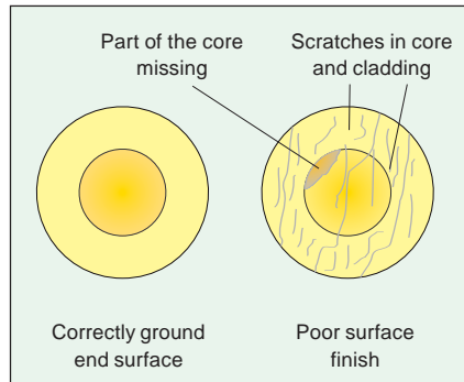
Fig. 8-14 A poorly finished end surface results in increased splice loss.
