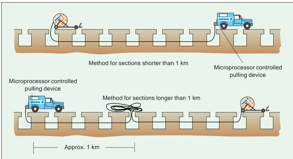
Fig. 11-11 Suitable methods of cable laying in ducts.
