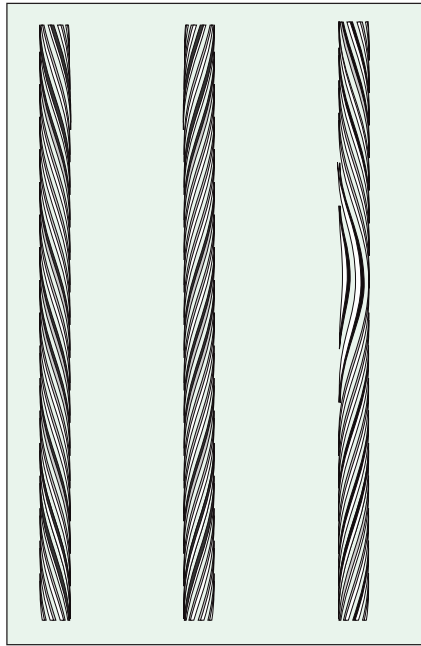
Fig. 5-23 Slotted core profiles. From left to right S, Z and SZ stranding.
