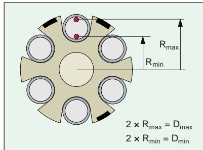
Fig. 5-26 The fiber can move freely between R_{max} and R_{min} in an optical fiber cable with a slot profile.
