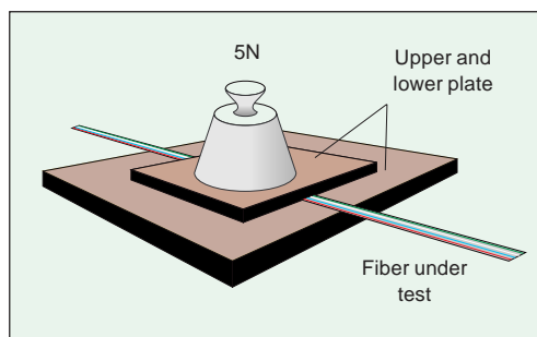
Fig.5-13 Setup for crush test.
