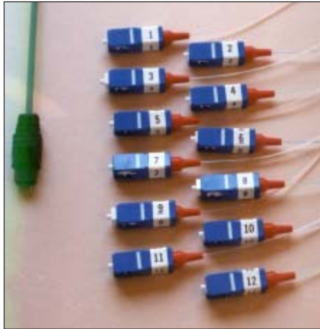
Fig. 8-42 Comparison between the 12-fiber MT-connector representing the ribbon technology and twelve SC-connectors representing the single fiber technology
