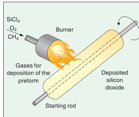
Fig. 3-7 The OVD method for making a preform.
