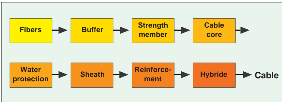
Fig. 5-1 General outline of the parameter involved in choosing the right optical fiber cable design.
