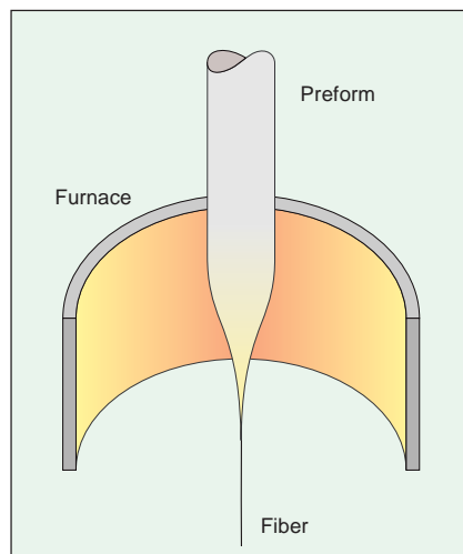
Fig. 3-9 Fiber drawing.
