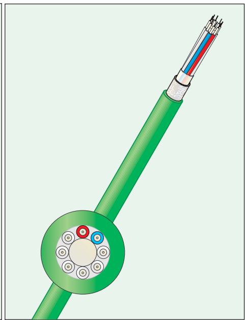
Fig. 5-22 Optical fiber cable; concentric construction with tight buffered fibers around the central strength member. Cable illustrated is the GNHLBDUV
