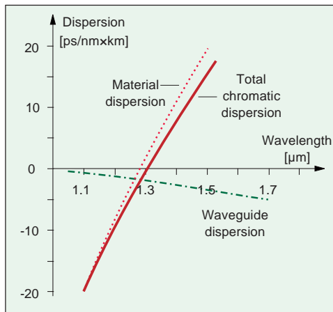
Fig. 9-8 The chromatic dispersion is the sum of material- and waveguide dispersion.
